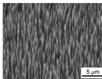
Figure 1. SEM image of vertically aligned diamond nanowires. [10]
